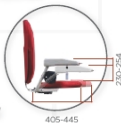
Detail 1 Armrests and seat adjustment.
